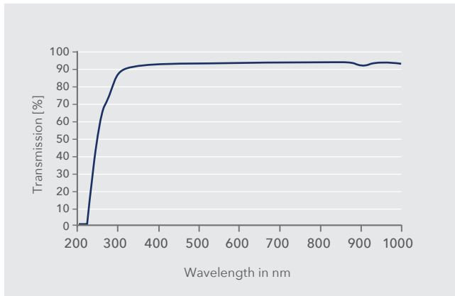
■ LSR 7070 (Thickness 2 mm)
