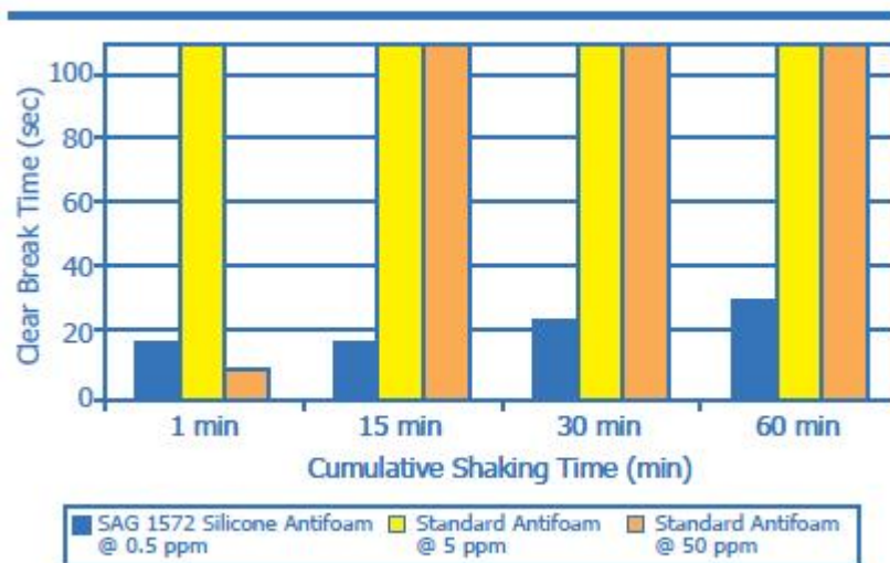
Figure 1: Antifoam Efficiency in 2.5% Glyphosate Formulation
